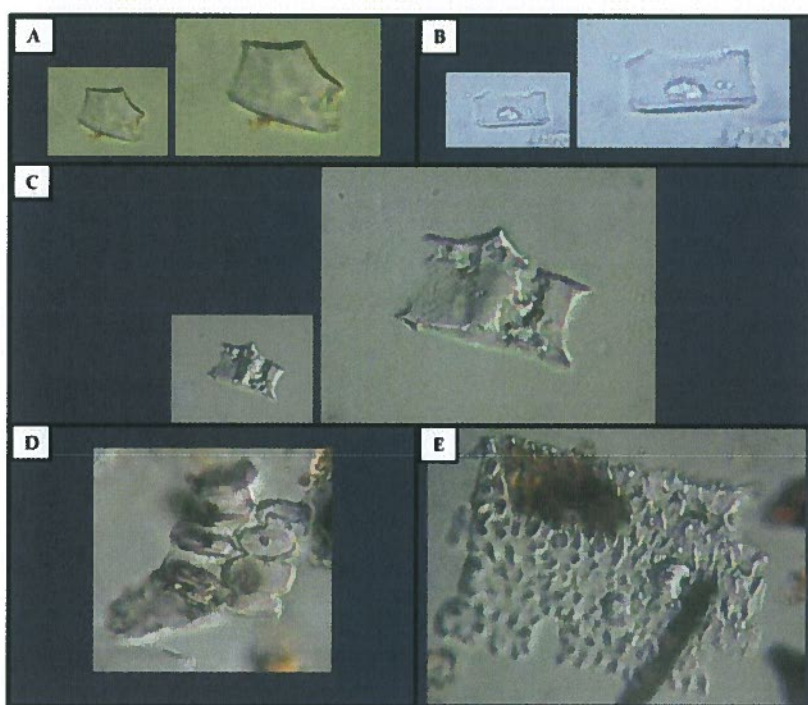
FIGURE 60. MICROGRAPH COMPILATION OF ZEa MAYS PHYTOLITHS RECOVERED FROM NEW MEXICO.
