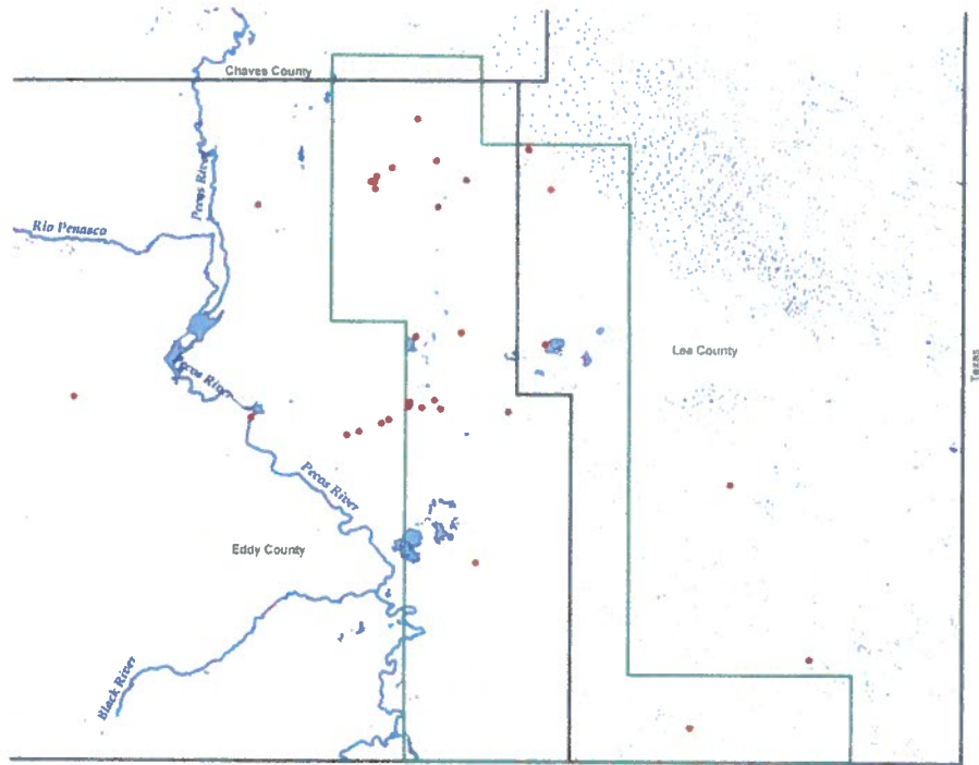
Figure 5. Map showing sites with evidence for corn ( Zea mays ) within the CFO boundaries (site LA 2000 not shown). Permian Basin PA boundary drawn in green. Streams and playas are shown in blue.
