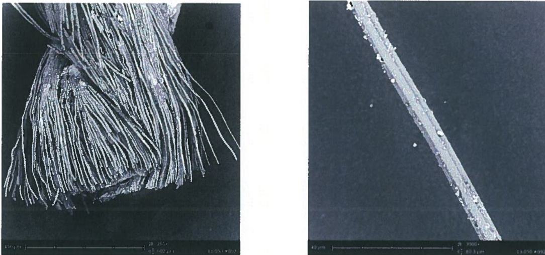
Figure 3. SEM micrographs of the serrated/cut end (left) and an individual fiber (right). Adapted from Scott Cummings and Kováčik 2012: Figure 34.
